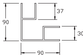
STANDARD 90° MULLION
