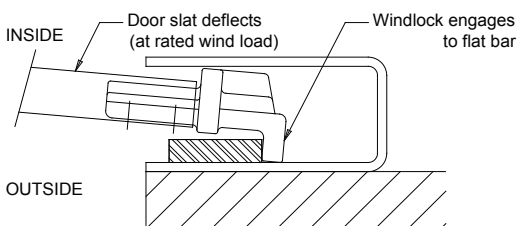
b: WINDLOCK AT RATED WINDLOAD
