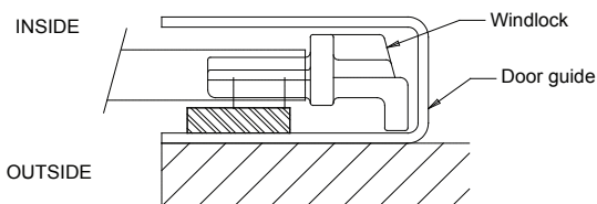
a: WINDLOCK AT NORMAL POSITION
