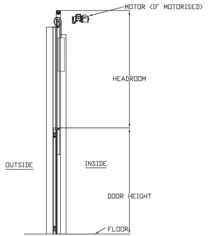
SECTION
