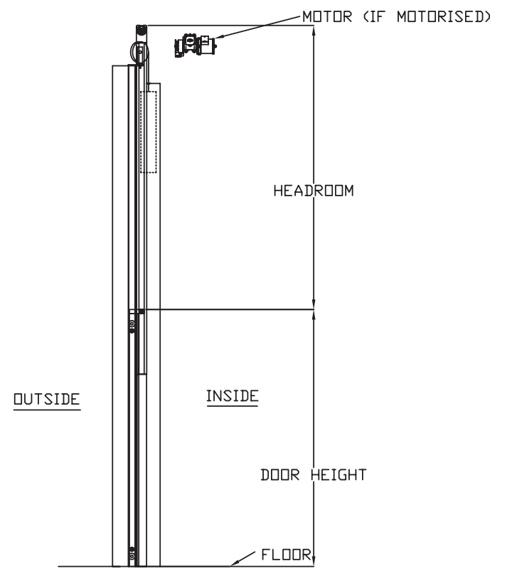
SECTION
