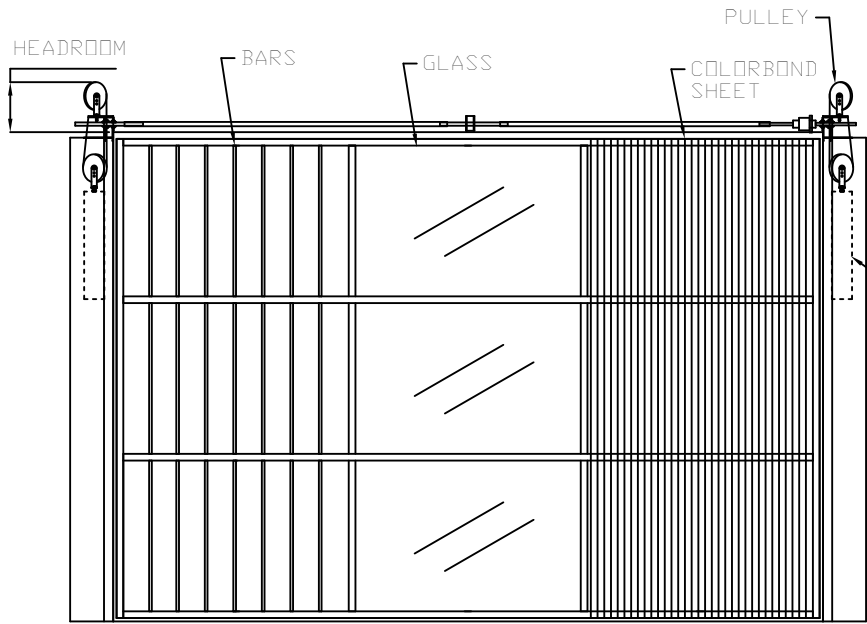
ELEVATION (INSIDE LOOKING OUT)
