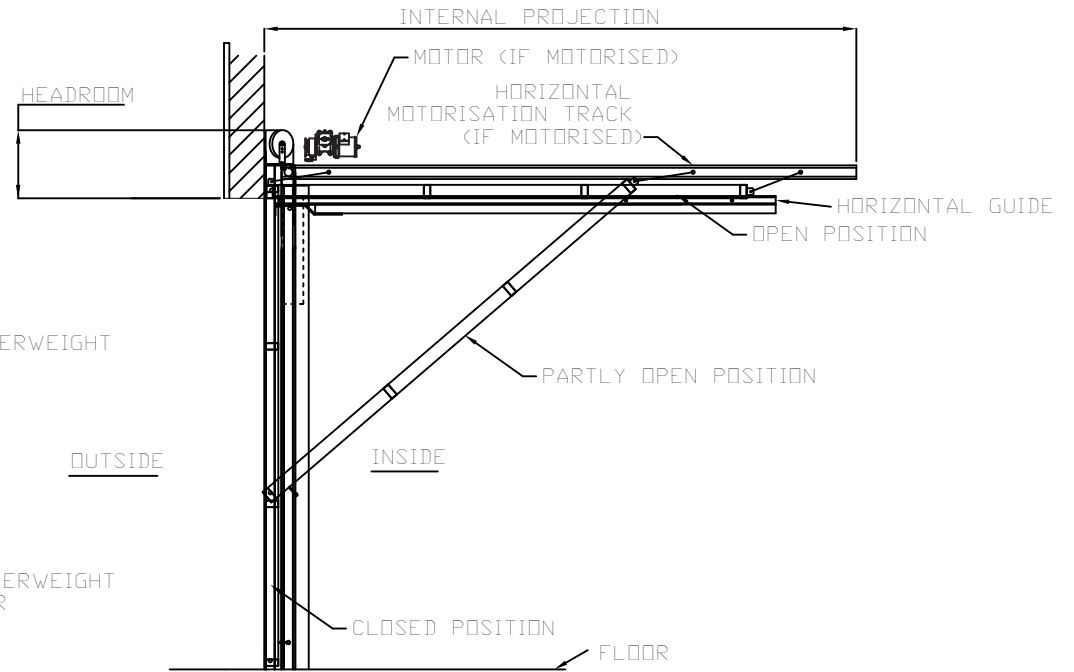
SECTION
