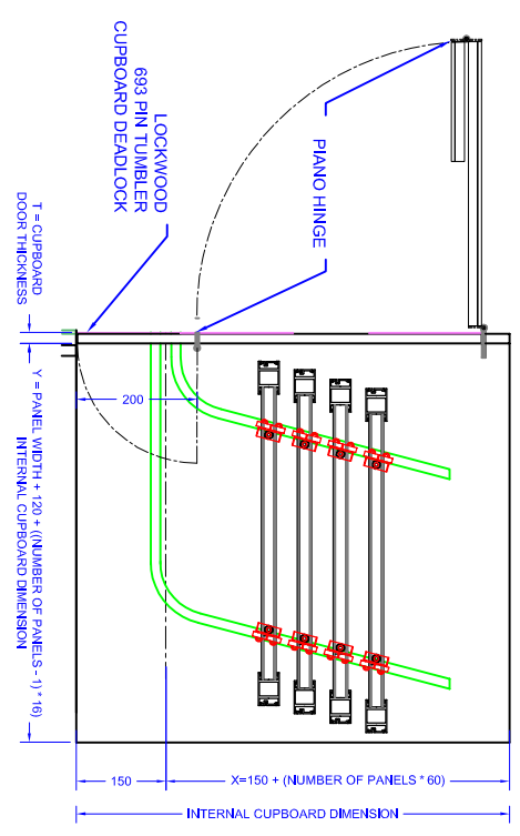
CUPBOARD DETAIL VIEW - INTERNAL CLEAR SIZES
