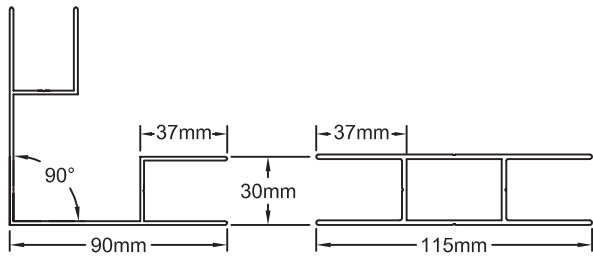
STANDARD 90° CORNER MULLION
