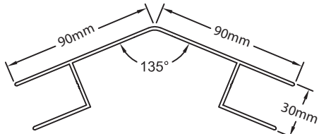
STANDARD 135° GUIDE
