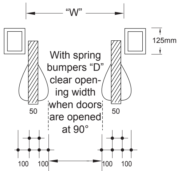
“Detail when using Spring Bumpers (Tear Drop)”
