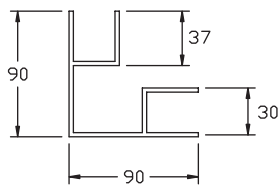
STANDARD 90° MULLION
