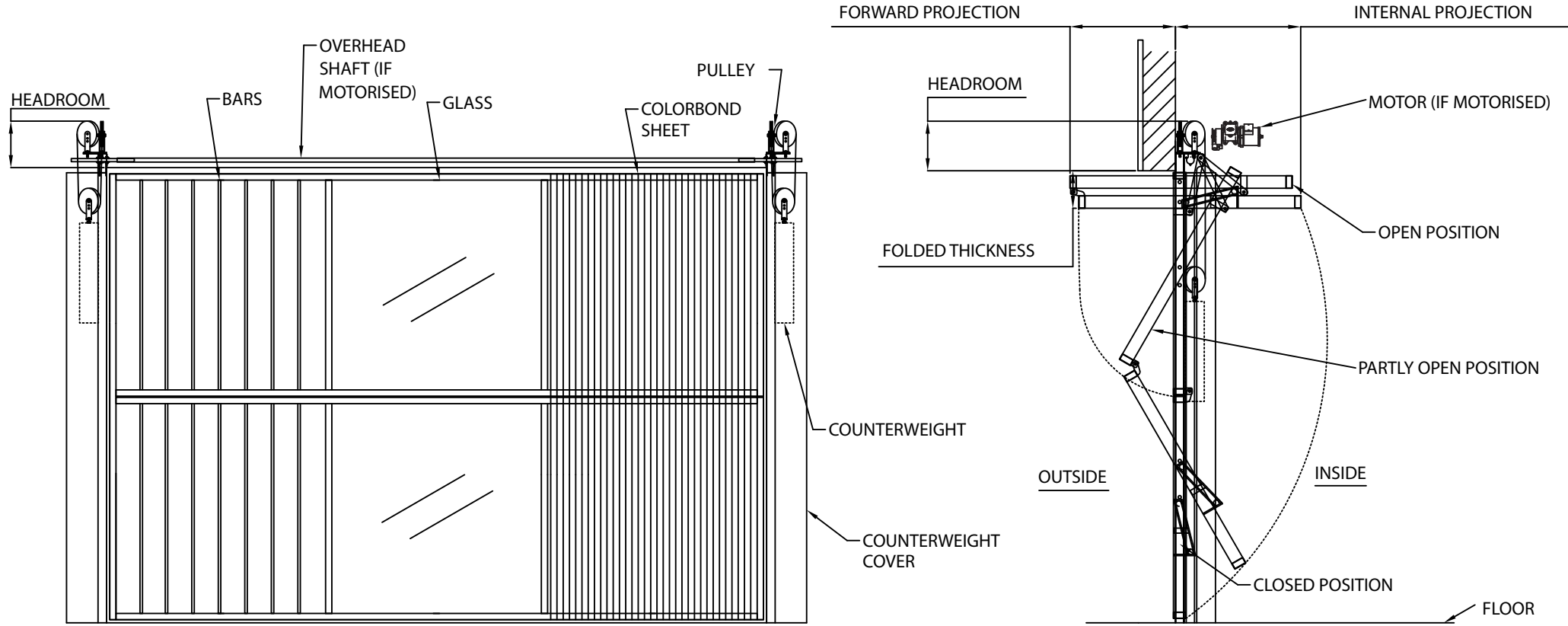
ELEVATION (INSIDE LOOKING OUT)
