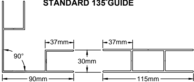
STANDARD 90° CORNER MULLION
