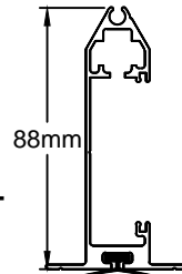
OPTIONAL EXTRA Black Rubber Bottom Rail Seal
