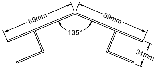
STANDARD 135° GUIDE
